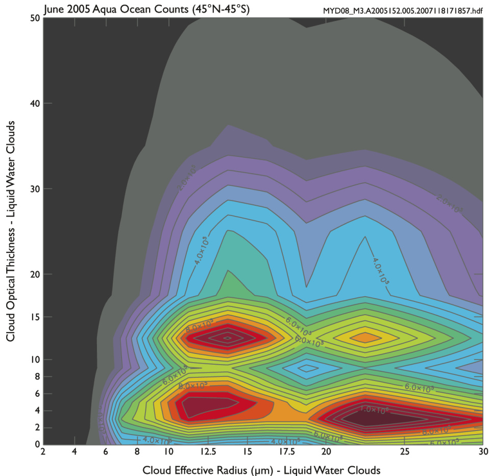
Figure 29. A June 2005 MYD08_M3 Counts Joint Histogram of cloud optical thickness (y-axis) vs. cloud effective radius (x-axis) for liquid water clouds displayed as a “colored contour plot” with post-processing to limit the data to ocean-only L3 grid cells that range from 45°N to 45°S. The top bin of cloud optical thickness from 50 to 100 was chopped off. The contour colors represent the number of counts in each bin (low is grey, high is red). Contour plots show a distorted (smoothed) view of the data stored in the joint histogram.
