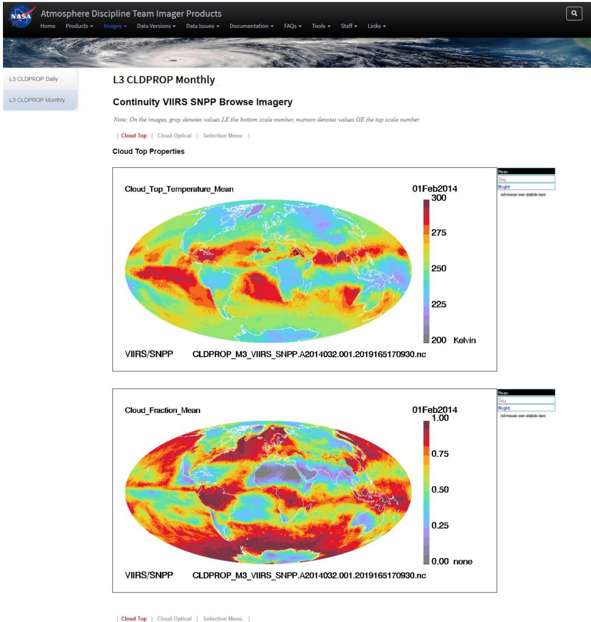
Figure 25. A capture of the Images > Continuity > L3 CLDPROP Monthly page. Here, users can find browse images for L3 CLDPROP Products. A JavaScript mouse-over feature allows one to view a number of different images in a single frame, allowing for quick ( flash ) a-b-c comparisons.
