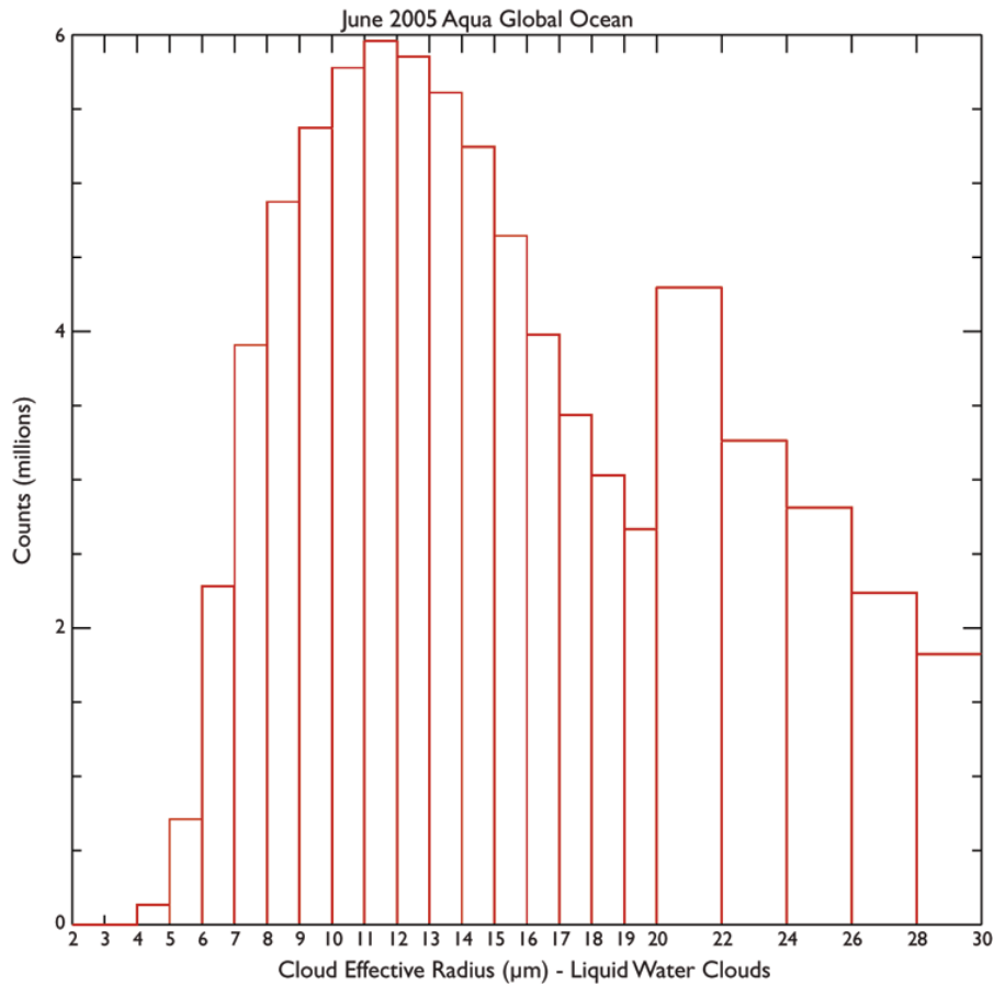
Figure 26. Marginal Histogram of L2 Pixel Counts (sampled) for Liquid Water Cloud Effective Radius during June 2005 (daytime only) for Global Ocean data from MODIS Standard Aqua/MODIS.
