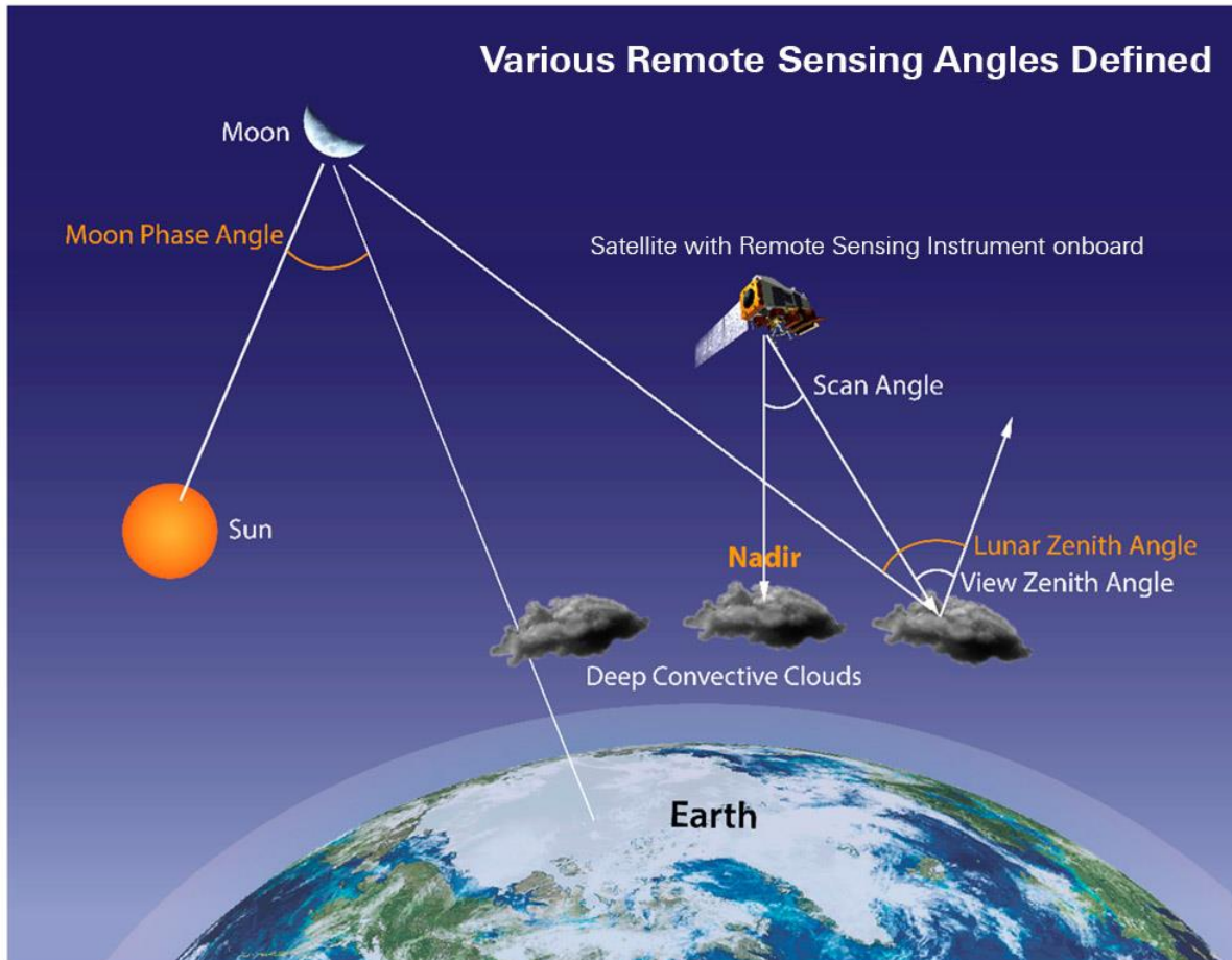
Figure 20. Abstract image (obviously not anywhere close to scale) providing a visual reference of various remote sensing angle definitions. The two key angles being discussed here are Scan Angle and View Zenith Angle. The L3 CLDPROP code limits L2 input to pixels where View Zenith Angle \leq 65.5^\circ , which primarily impacts VIIRS data.
