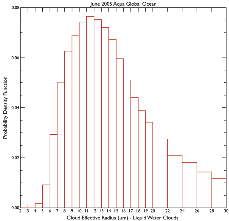
Figure 27. Marginal Histogram of Normalized Probability Density Function (PDF) (sampled) for Liquid Water Cloud Effective Radius during June 2005 (daytime only) for Global Ocean data from Aqua/MODIS.
