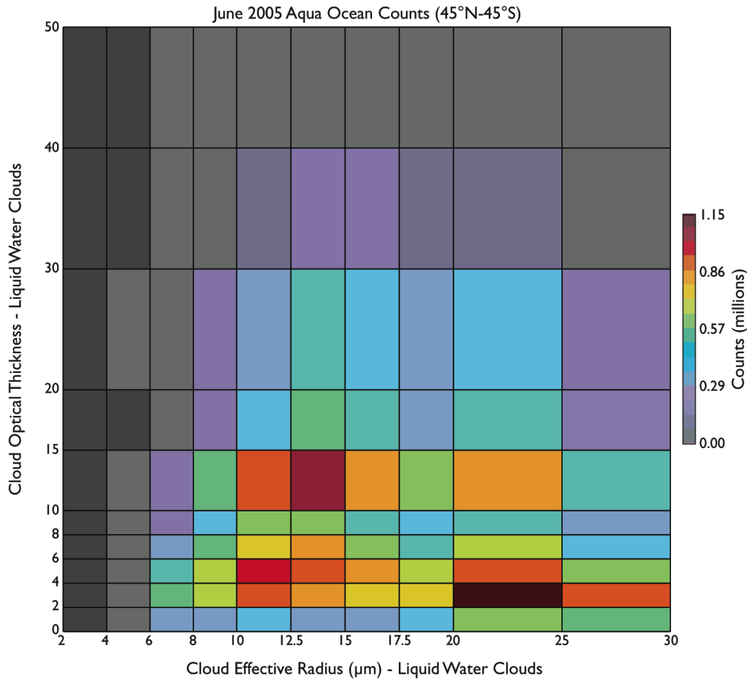
Figure 30. A June 2005 MYD08_M3 Counts Joint Histogram of cloud optical thickness (y-axis) vs. cloud effective radius (x-axis) for liquid water clouds displayed as a “colored histogram bin plot” with post-processing to limit the data to ocean-only L3 grid cells that range from 45°N to 45°S. The top bin of cloud optical thickness from 50 to 100 was chopped off. The bin colors represent the number of counts in each bin (low is grey, high is red).
