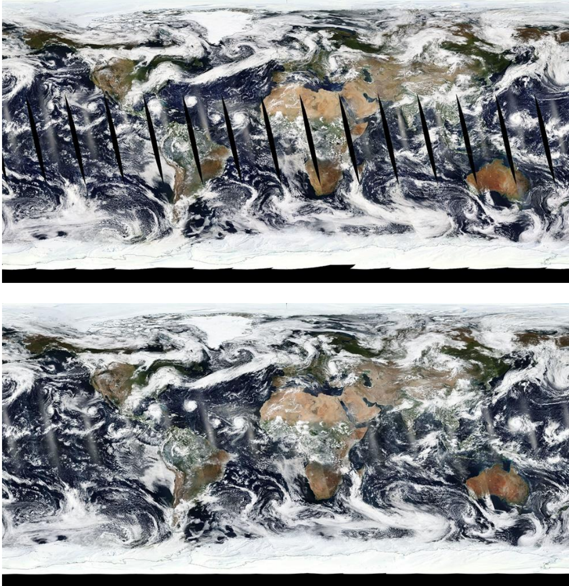
Figure 12. True color corrected reflectance (RGB:143) from September 10, 2018. (a) MODIS Aqua. (b) VIIRS SNPP. The vertical black strips over the tropics in the Aqua-MODIS image (top) are the gaps between MODIS swaths from successive orbits. Note that the VIIRS image does not have these orbital gaps due to its wider swath. Images courtesy of NASA Worldview.
