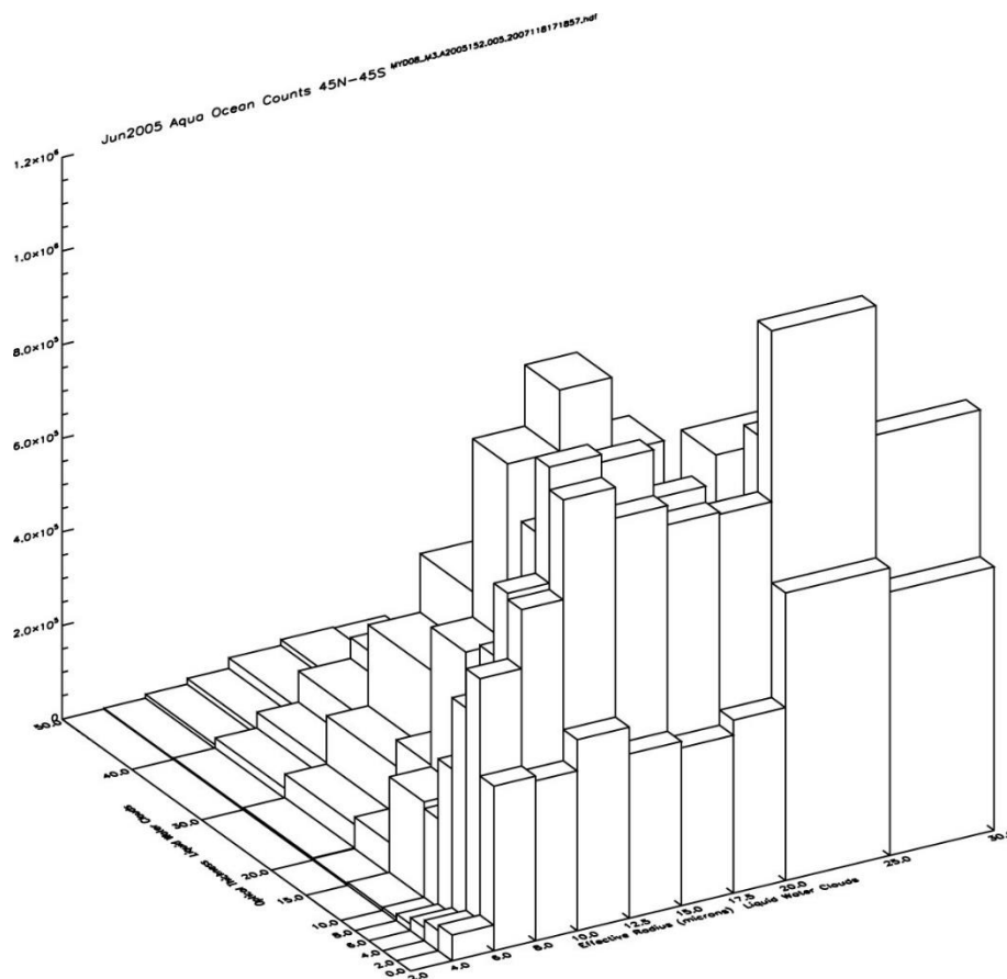
Figure 28. A June 2005 MYD08_M3 Counts Joint Histogram of cloud optical thickness (y-axis) vs. cloud effective radius (x-axis) for liquid water clouds displayed as a “3D lego plot” with post-processing to limit the data to ocean-only L3 grid cells that range from 45°N to 45°S. The top bin of cloud optical thickness from 50 to 100 was chopped off. The height of each Lego bar represents the number of counts in each bin. It is often difficult to impossible to orient lego plots to make all bins visible.
