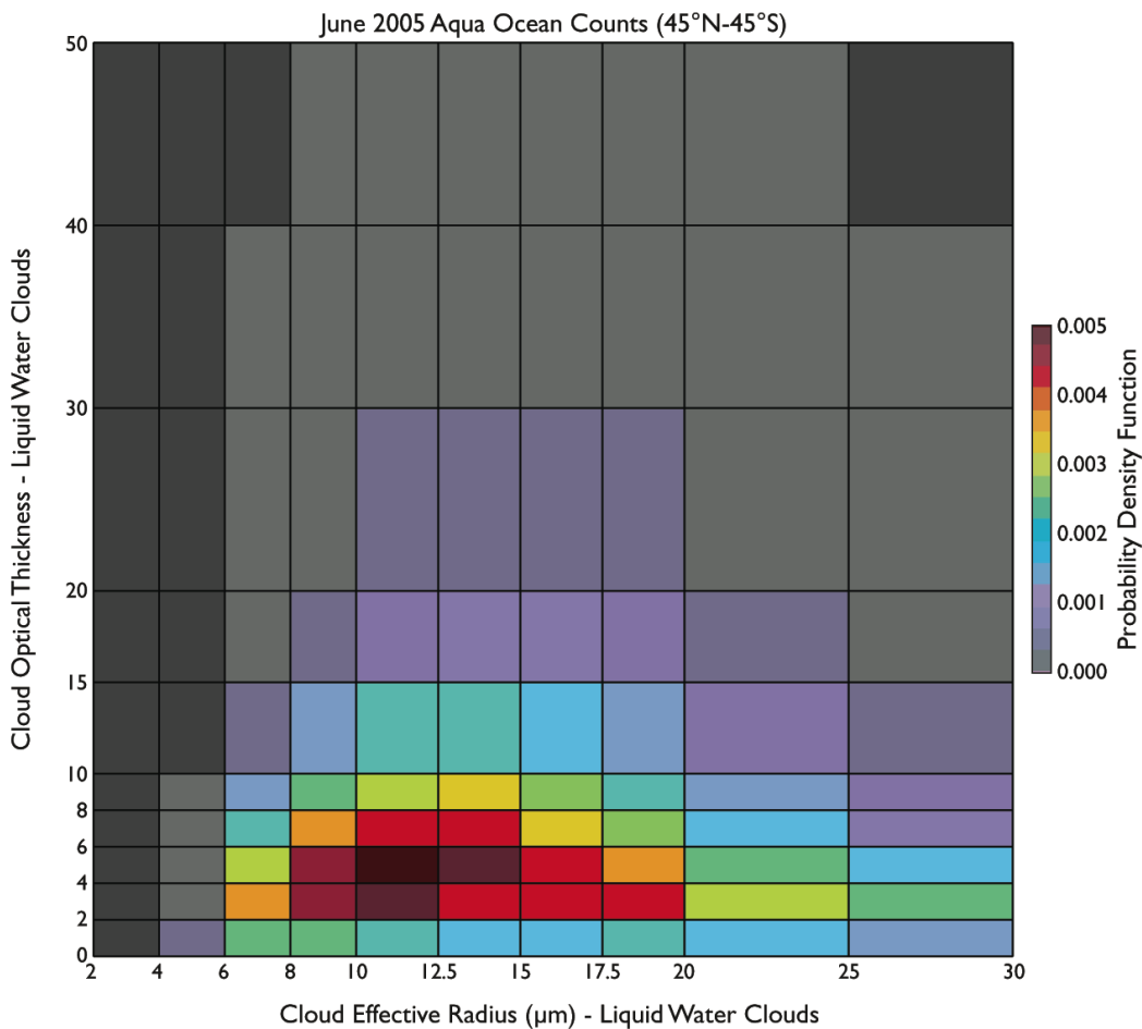
Figure 31. A June 2005 MYD08_M3 Normalized Probability Density Function (PDF) Joint Histogram of Cloud Optical Thickness (y-axis) vs. Cloud Effective Radius (x-axis) for Liquid Water Clouds displayed as a “colored histogram bin plot” with post-processing to limit the data to Ocean-only L3 grid cells that range from 45N to 45S. The top bin of Cloud Optical Thickness from 50 to 100 was removed. The bin colors represent the PDF in each bin (low probability is grey, high probability is red).
