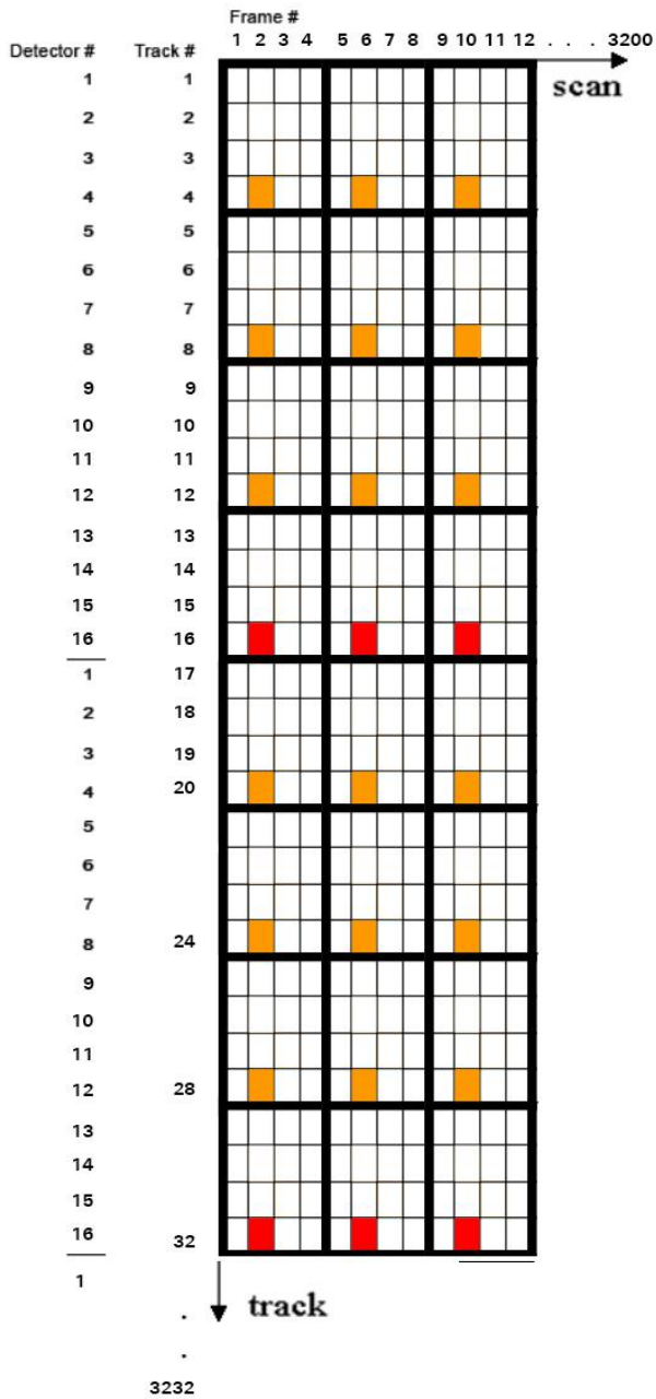
Figure 14. Illustration of the Sampling Technique used on L2 750m VIIRS data when computing L3 statistics. The orange grids are the sampled grids that are used in L3. The red grids are (regularly) sampled grids that are later set to fill-value in the L3 code, so that lower quality data (from VIIRS detector 16) is not aggregated into L3.
